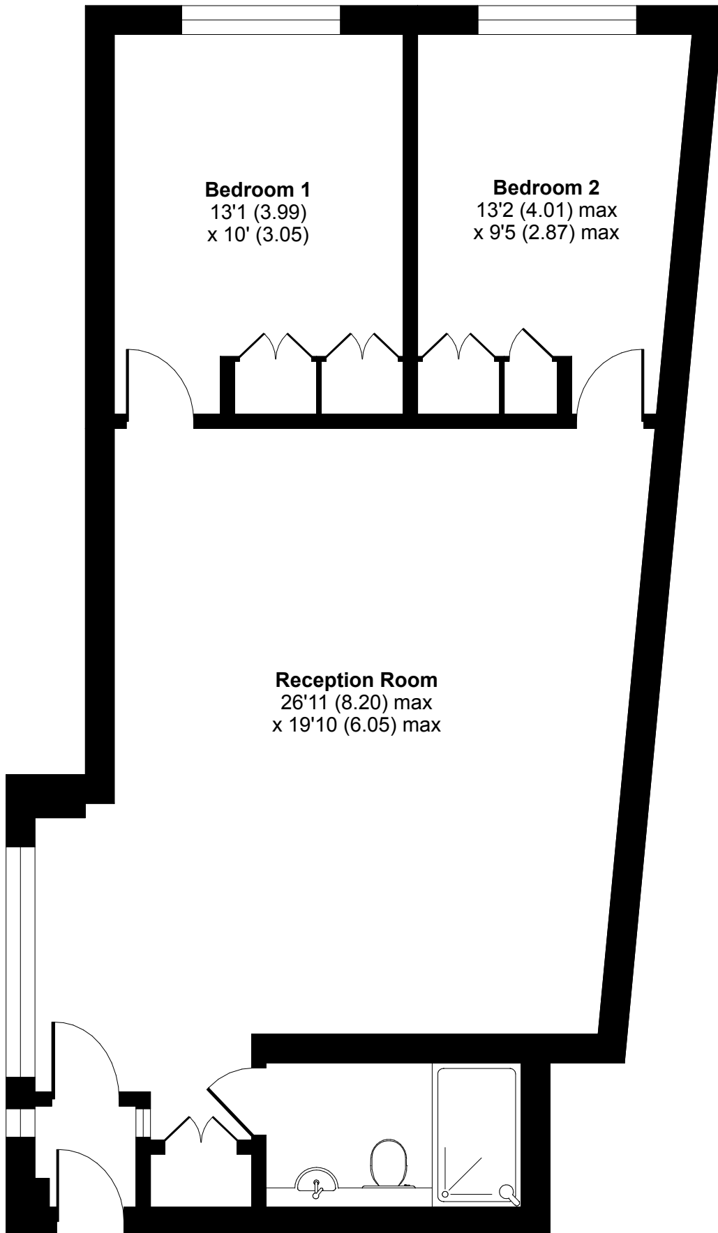
GROUND FLOOR
